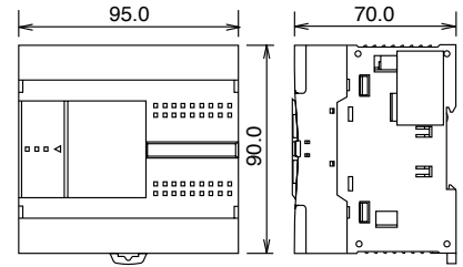
FC5A-C24R2, FC5A-C24R2C
