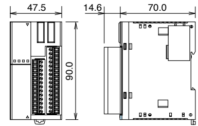
FC5A-D16RK1, FC5A-D16RS1
